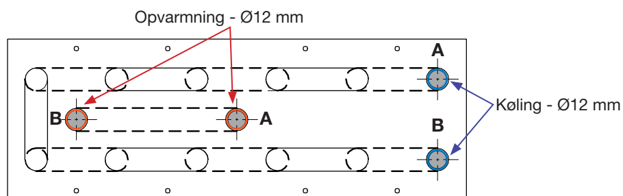
Figur 4. Fasadium: 1000, 1200, 1500.
